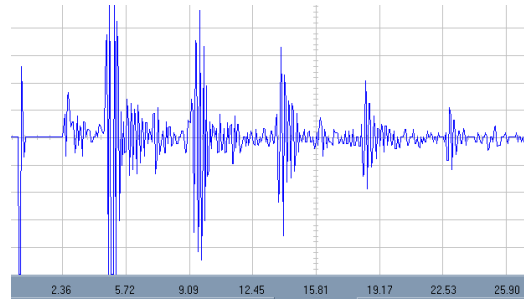
Figure 1. Pulse-echo flaw detection, ref [1] Figure 2. Results using mm-scale PZT specimen
