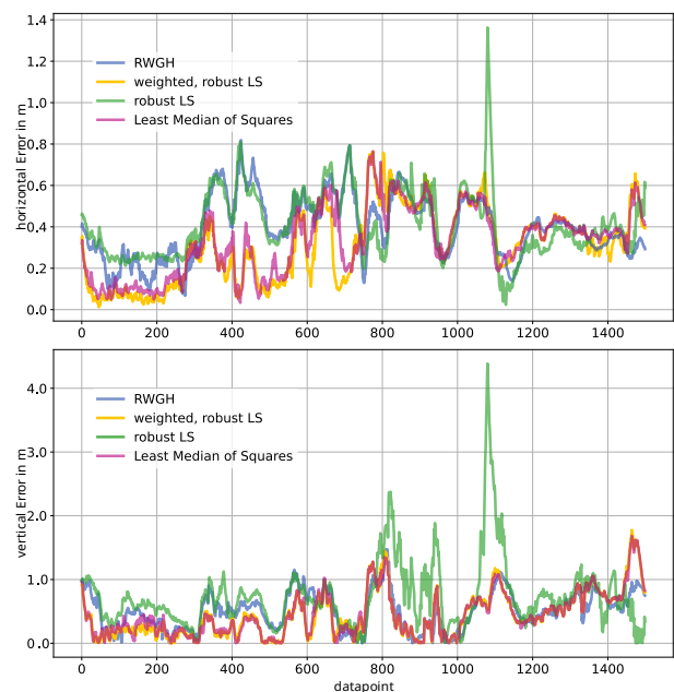
Figure 6. Excerpt of horizontal and vertical positioning errors over a continuous dynamic trajectory
