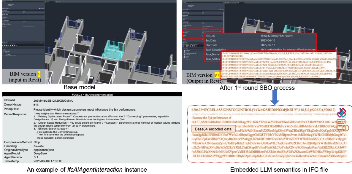
Figure 7. Embedded LLM Agent-enhanced SBO semantics in IFC
