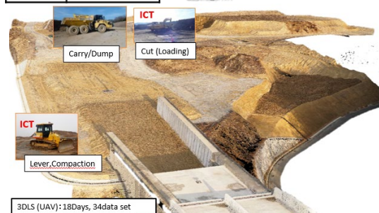
Figure 7. Site-C Outlines(upper) and Point cloud by LS with UAV
