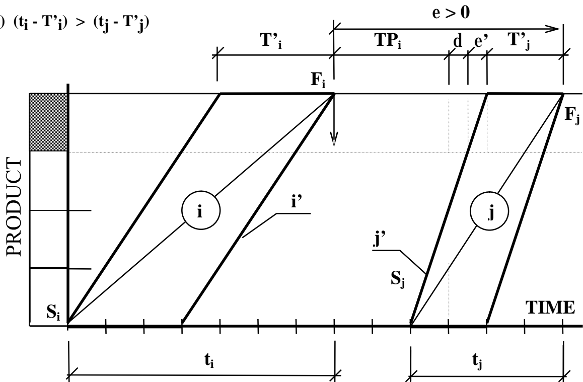
Figure 2: Principle of the construction technology link
