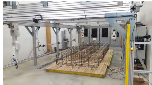
Figure 1. Gantry robot system.
