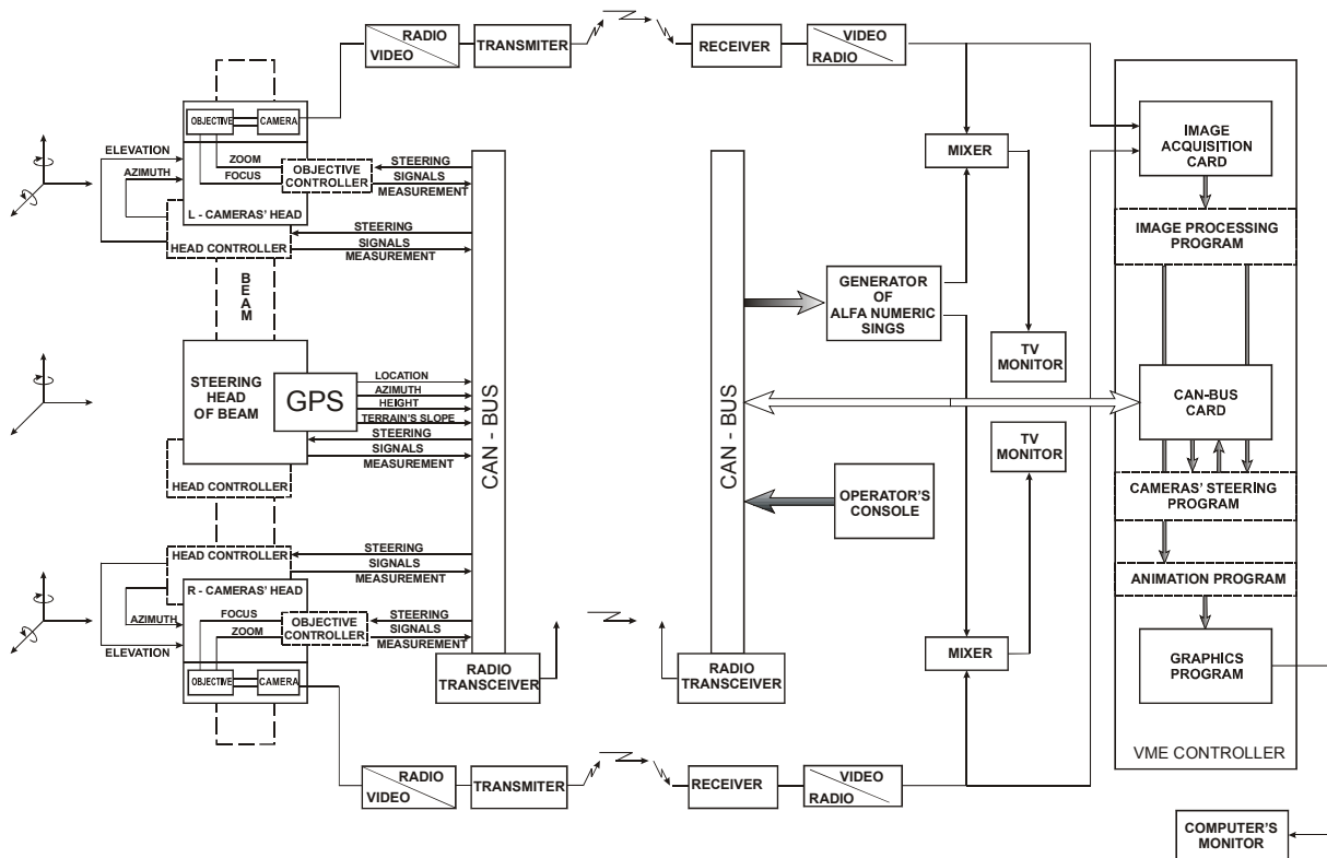
Figure 3. Scheme of vision system
