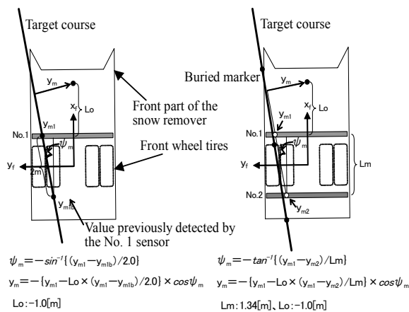
Figure 3. Lane Marker Sensor Guidance Method
