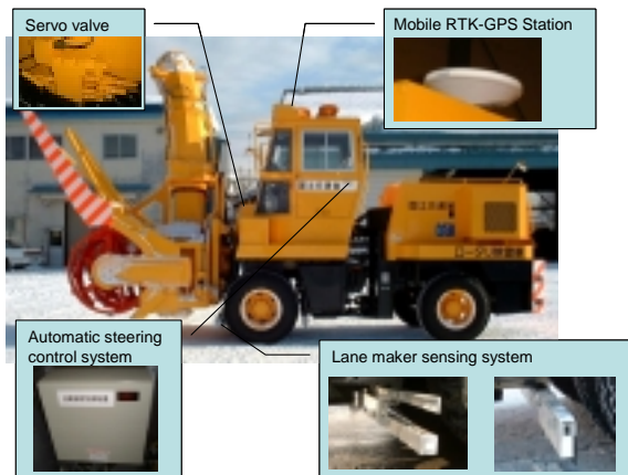
Fig. 6 Rotary Snow Remover Equipped with an Automatic Steering Support Function
