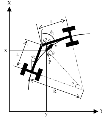
Figure 1. Coordinate System (Model of a Snow Remover)
