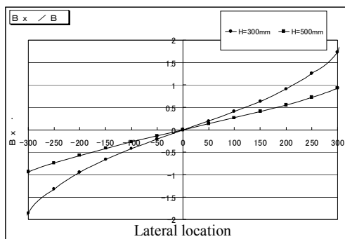
Figure 4. B_x/B_z Relationship
