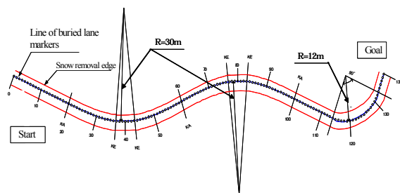
Figure 7. Layout of the Test Course
