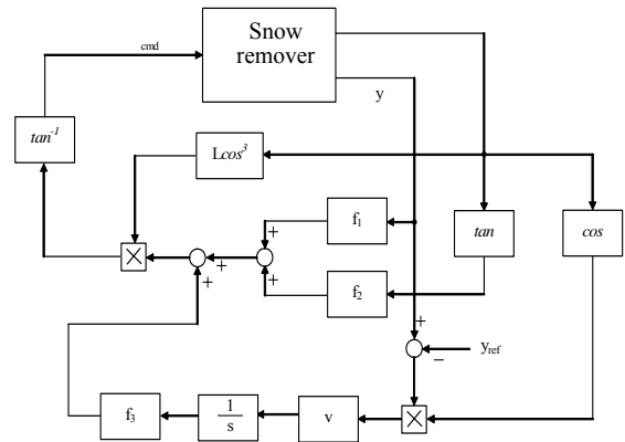
Figure 2. Integrated Servo System Control Block Diagram
