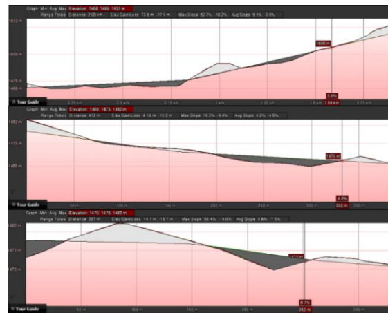
Figure 4. Three Road Segments Elevation Profiles and Vertical Alignments
