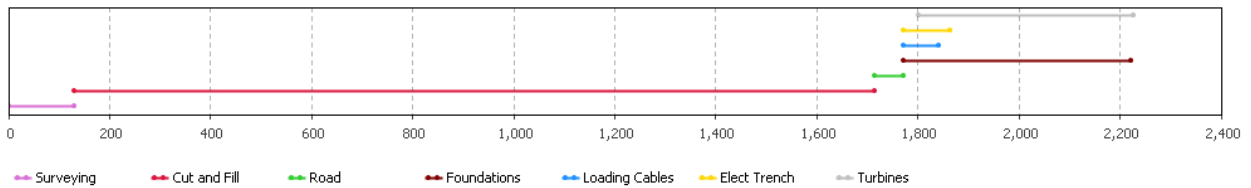
Figure 6. Gantt chart of the Falougha's Wind Farm Construction Process (in working days)
