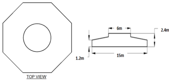
Figure 5. Turbine Foundation Dimensions
