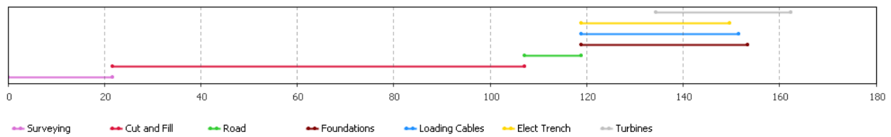
Figure 8. Optimized Gantt chart of the Falougha's Wind Farm Construction Process (in working days)
