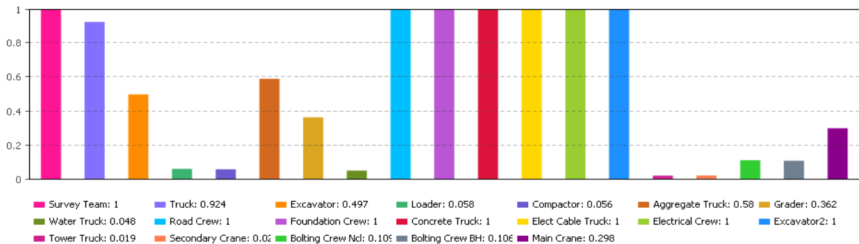
Figure 7. Resource Utilization Rates of the Falougha Wind Farm Project
