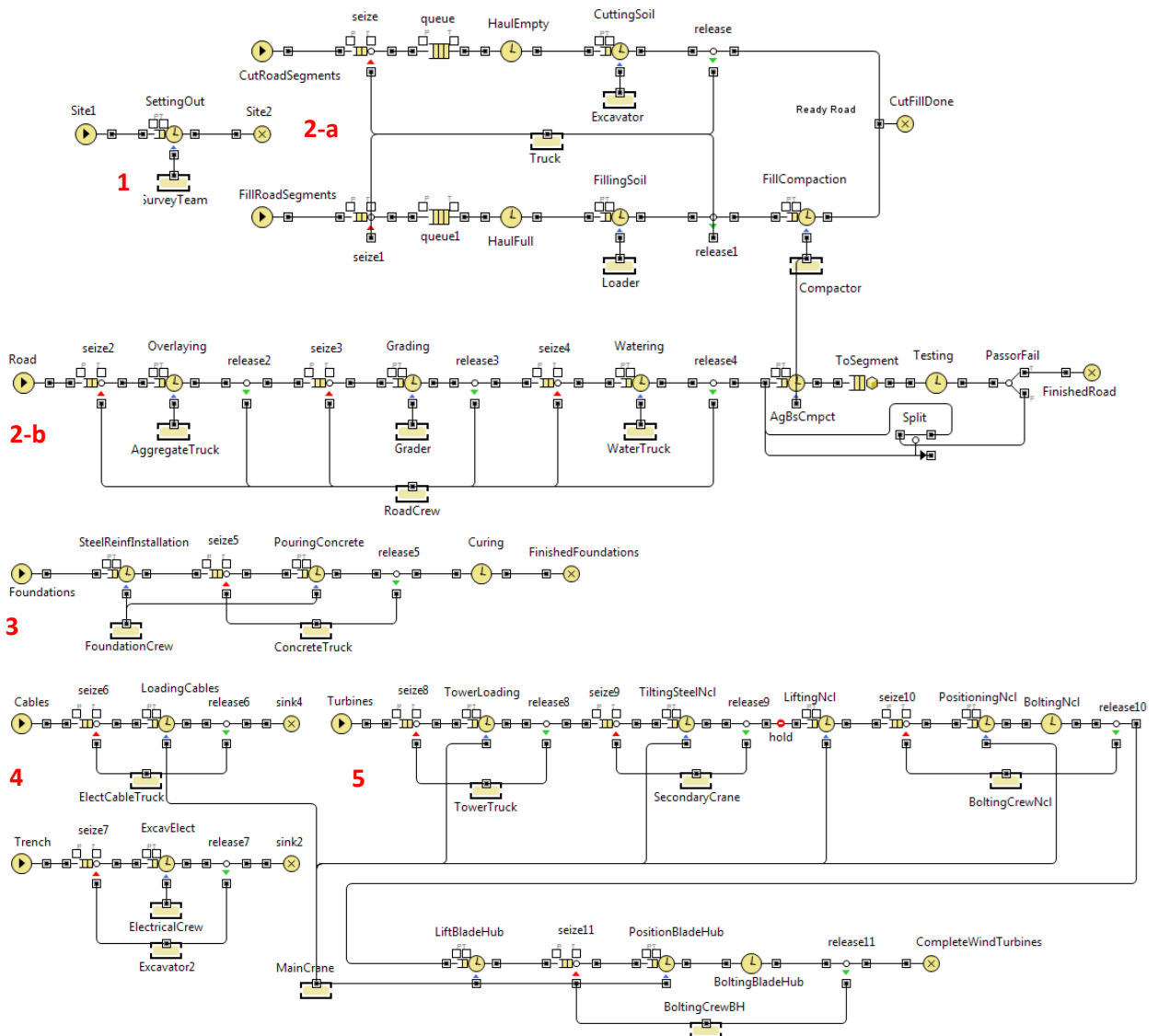
Figure 2. AnyLogic Model of the Construction Process
