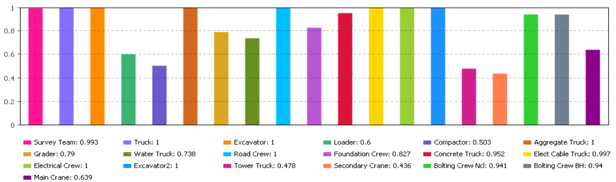
Figure 9. Optimized Resource Utilization Rates of the Falougha Wind Farm Project
